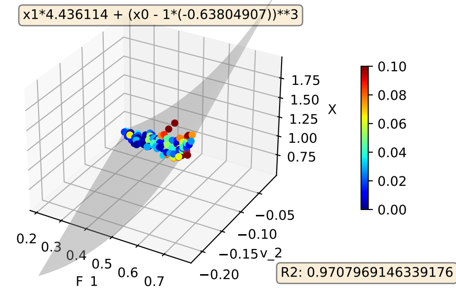
XBeamEnergy400TestSize0.5try 1 Model:3D
