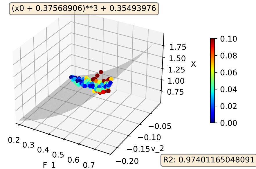
XBeamEnergy400TestSize0.05try 0 Model:3D
