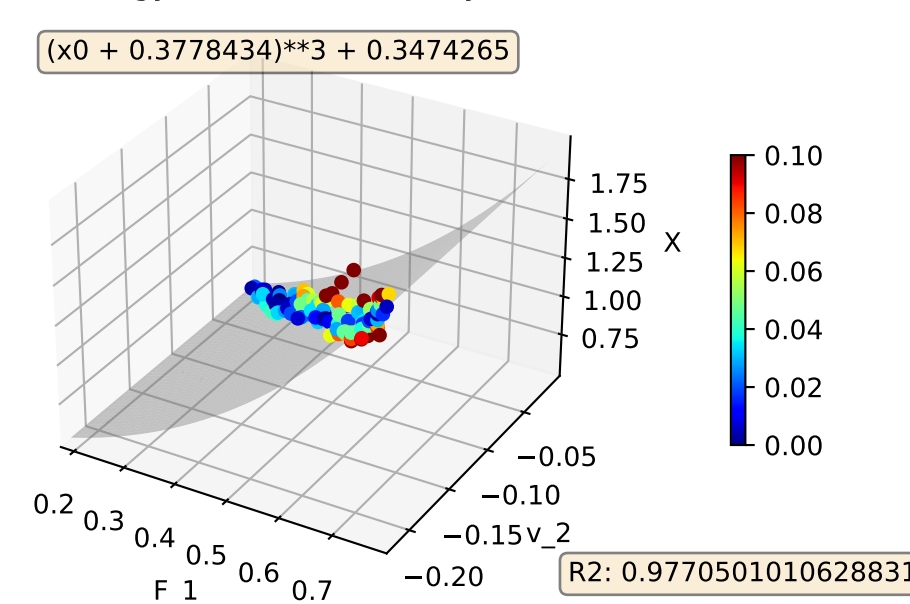
XBeamEnergy400TestSize0.25try 4 Model:3D
