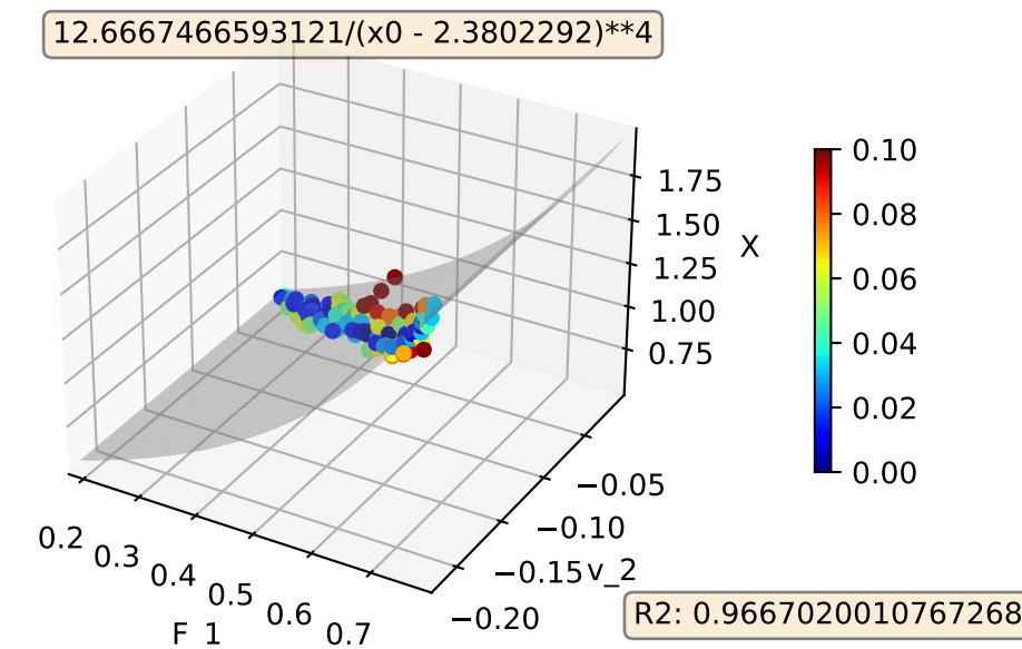
XBeamEnergy400TestSize0.1try 2 Model:3D
