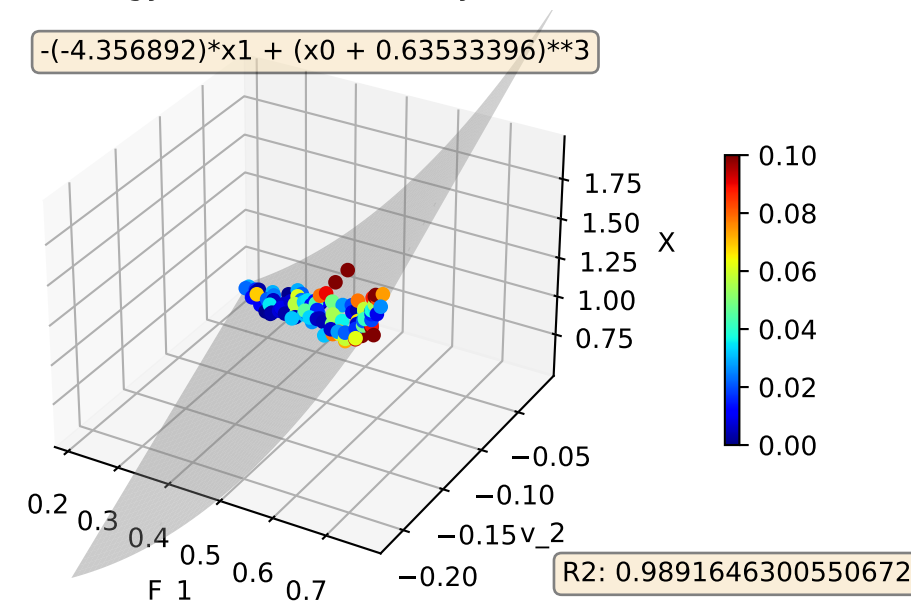
XBeamEnergy400TestSize0.15try 0 Model:3D
