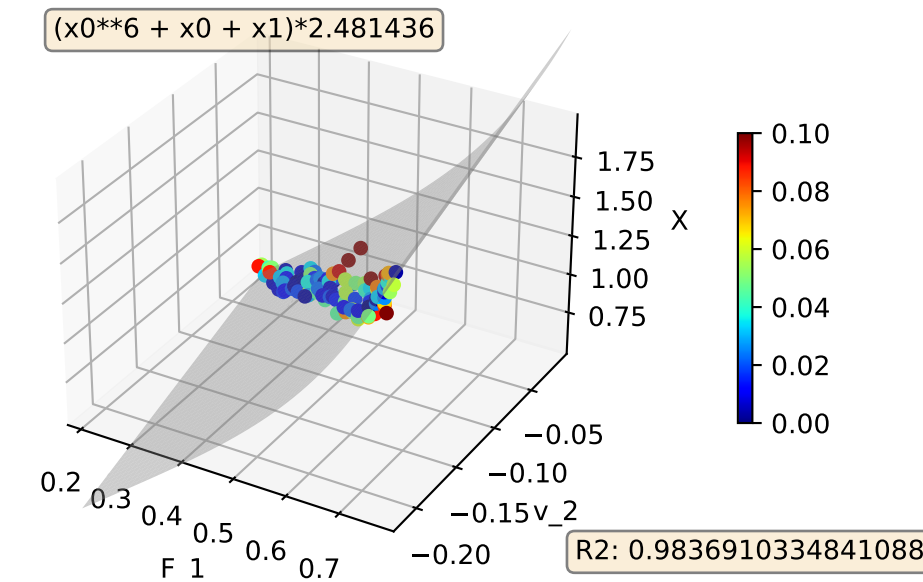
XBeamEnergy400TestSize0.05try 3 Model:3D
