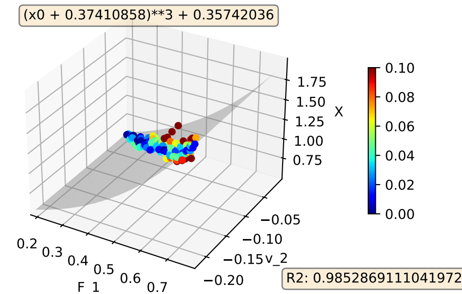
XBeamEnergy400TestSize0.1try 0 Model:3D
