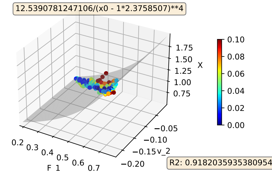
XBeamEnergy400TestSize0.05try 4 Model:3D
