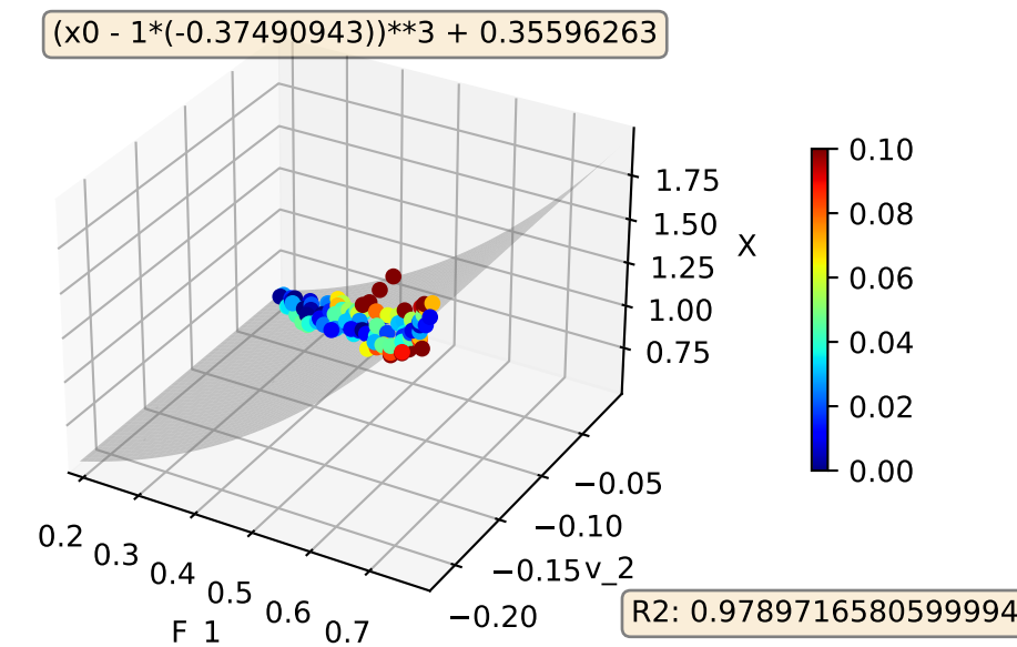
XBeamEnergy400TestSize0.1try 3 Model:3D
