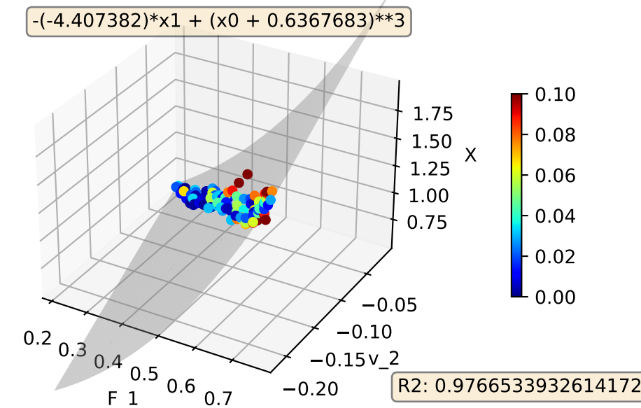
XBeamEnergy400TestSize0.1try 4 Model:3D
