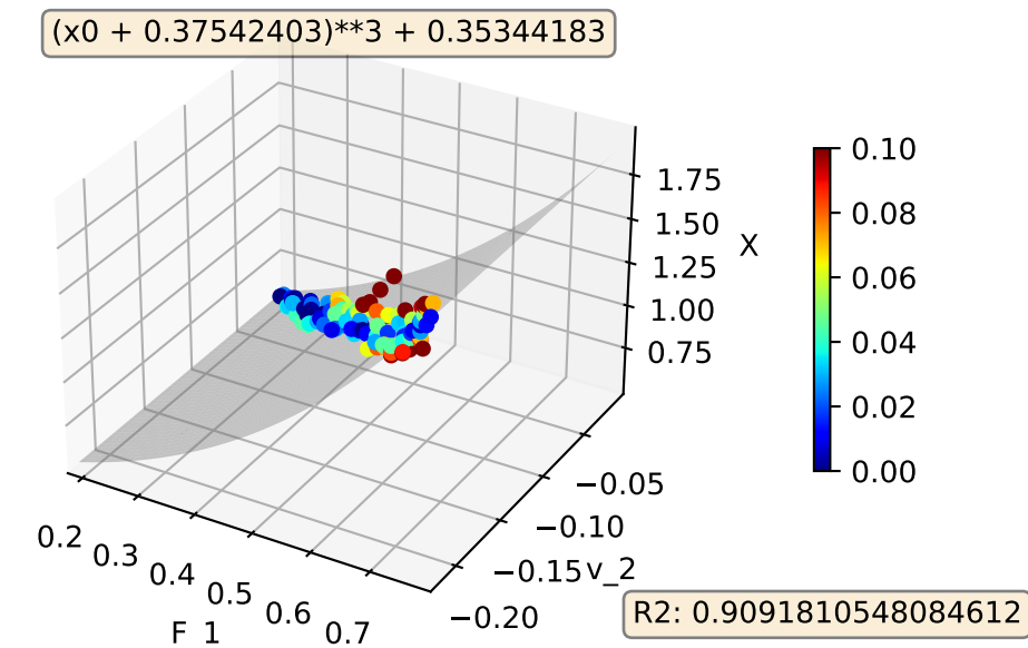
XBeamEnergy400TestSize0.05try 1 Model:3D
