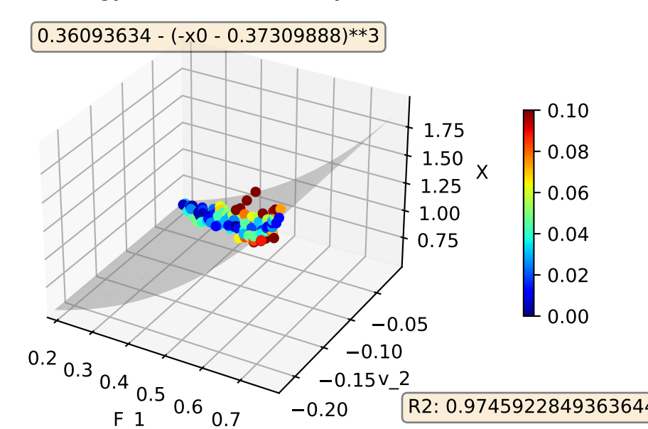
XBeamEnergy400TestSize0.15try 4 Model:3D
